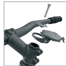
Mounting alternative 2
