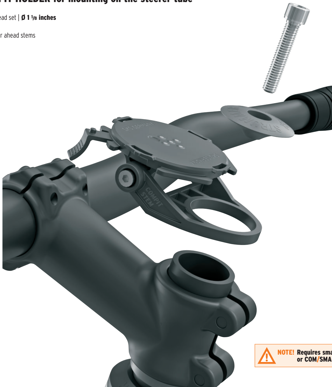
Mounting alternative 1
